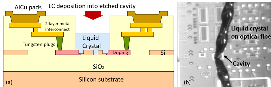
Figure 1. (a) Integration of liquid crystal in iSiPP50G platform (b) Experimental deposition of liquid crystal in etched cavity, using a motorized cleaved fiber as delivery mechanism
