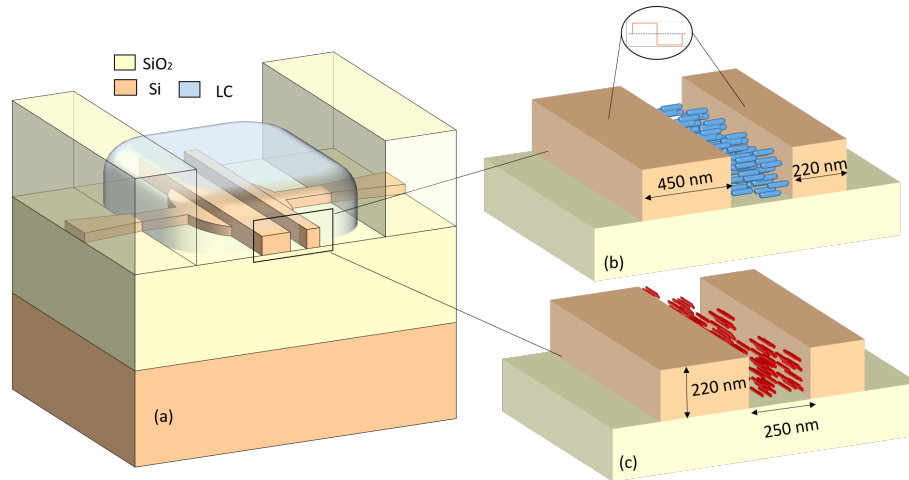
Figure 2. Operation principle of the phase shifter. (a) a shifter with an etched opening with a droplet of liquid crystal, accessed by silicon which is electrically connected to the oxide-clad back-end. (b) LC molecules oriented when a voltage is applied. (c) LC molecules relaxed along the waveguide when no voltage is applied.
