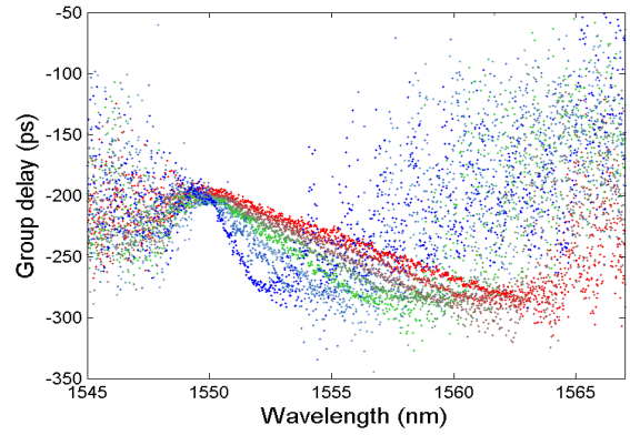
Figure 5. Group delay of linearly chirped Bragg gratings with chirp rates of 2.8 - 14.4 nm/cm
