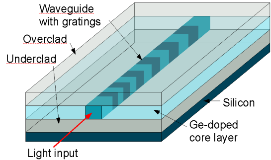
Figure 1. A DGW buried channel waveguide with integral chirped Bragg grating
