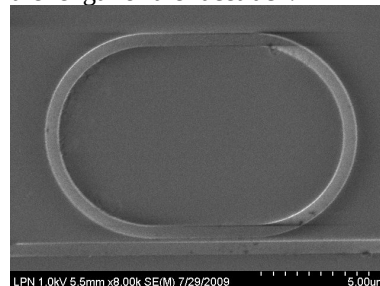
Figure 1. SEM image of racetrack resonators
