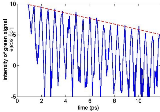
Figure 2. The intensity of the signal measured at 540nm (log scale) vs the delay time of the pump. The temporal ring-down of the racetrack shown as a sequence of diminishing peaks.
