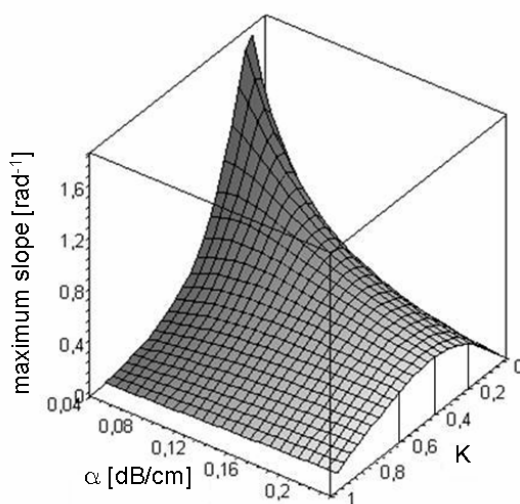
Fig. 5: Steepest slope of the ring resonances as function of the waveguide propagation losses \alpha and of the power coupling coefficient K of the directional coupler.
