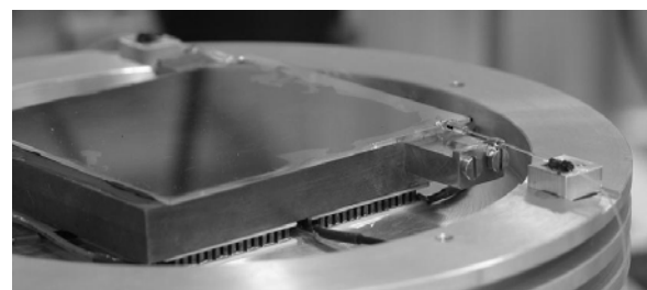
Fig. 6: Opened aluminum box with pigtailed ring resonator on a copper base plate, which can be temperature stabilized by a thermoelectric cooler/heater.
