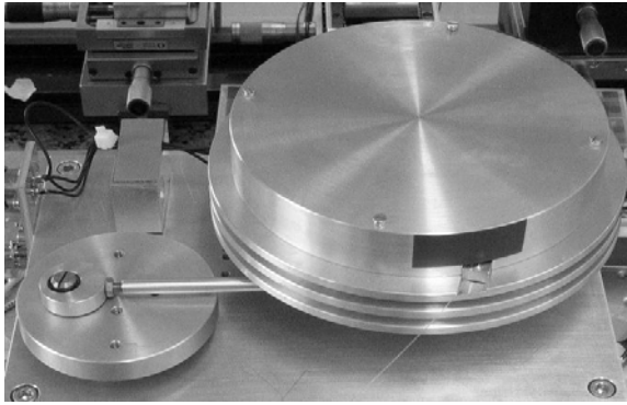
Fig. 7: Electromechanical drive to rotate the packaged ring resonator.
