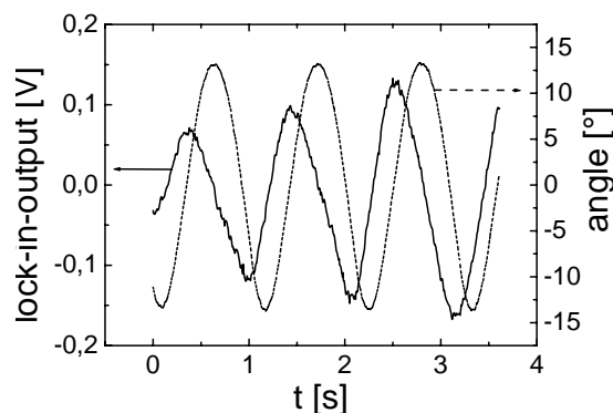
Fig. 10: Angular position of the ring resonator (right ordinate) and output signal of the lock-in amplifier (left ordinate) versus time. 0.1 V correspond to a rotation rate of about 100 \text{ }^\circ/\text{s} .
