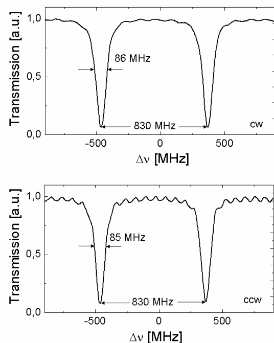
Fig. 9: Cw and ccw resonance curves of a ring resonator in bidirectional operation.
