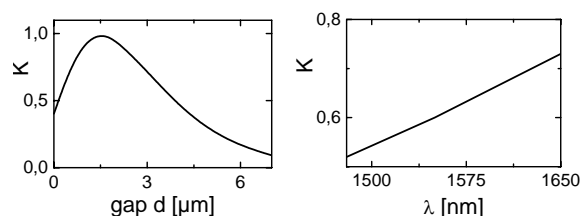
Fig. 3: Left: power coupling coefficient K as function of the minimum gap d of the directional coupler at \lambda = 1550 nm. Right: K versus wavelength for d = 4.9 \mu\text{m} .
