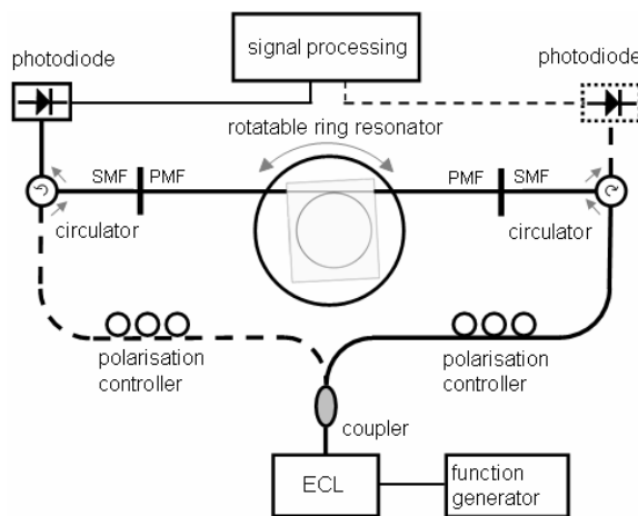
Fig. 8: Experimental setup to investigate the ring resonator and to study the Sagnac effect in uni- or bidirectional (dotted) operation. ECL: tunable extended cavity laser. PMF: polarization maintaining fiber. SMF: single-mode fiber
