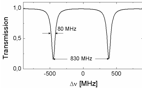
Fig. 4: Calculated straight waveguide transmission (see Fig. 1) versus a change \Delta\nu of the optical frequency for \alpha = 0.03 dB/cm and K = 0.3 .
