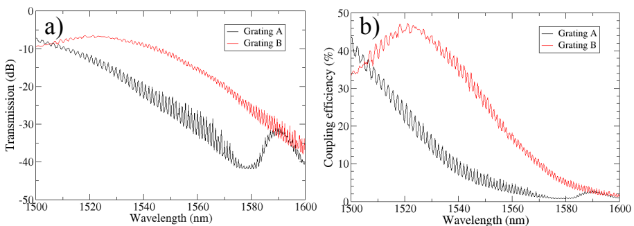
Fig. 2: a – Transmission through a 50 \mu m wire with two grating couplers, for two different grating; b – Corresponding coupling efficiency.
