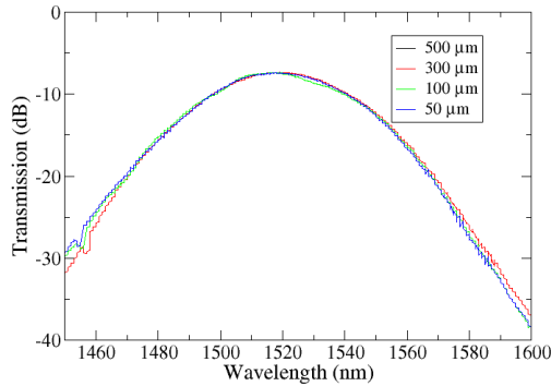
Fig. 3 : Transmission through 400nm wide wires of different lengths : 500 \mu\text{m} (black), 300 \mu\text{m} (red), 100 \mu\text{m} (green), and 50 \mu\text{m} (blue).
