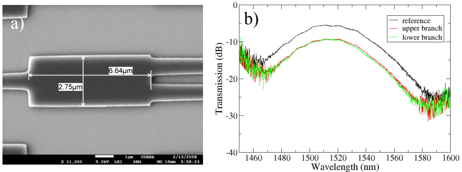
Fig.5 : a – SEM image of a fabricated MMI ; b – transmission through both output branches, together with the reference.
