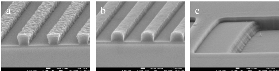
Fig 1: a – Resist pattern of a grating without post-bake; b – Same pattern after a 150°C post-bake for 2’; c – Shallow-deep transition morphology.
