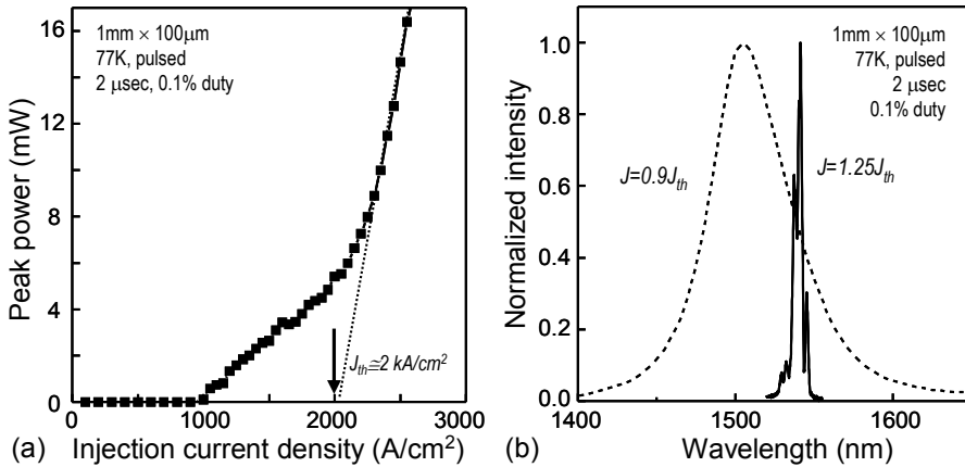
Fig. 2 (a) L-I curve of the fabricated laser devices at 77K under pulsed operation. (b) EL spectra above and below the threshold current density, J_{th} \approx 2 \text{ kA/cm}^2 .
