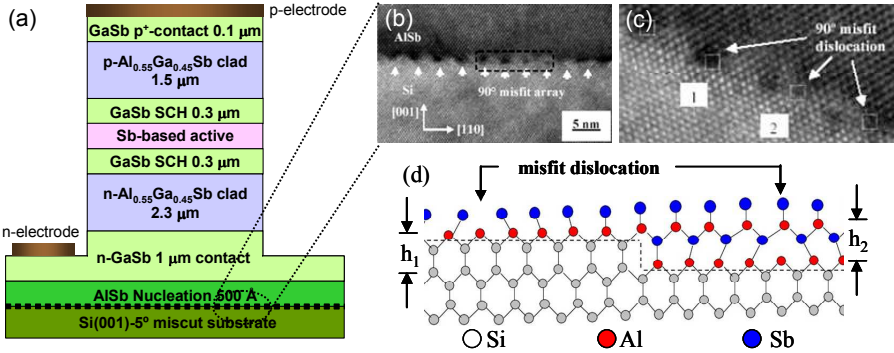
Fig. 1 (a) Schematic illustration of fabricated III-Sb based laser structures monolithically grown on 5^\circ miscut Si (001) substrates. (b) and (c) cross-sectional transmission electron microscope images of the interface between AISb and Si. (d) Schematic illustration of the IMF interface between AISb and Si.
