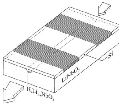
Fig.1. Sketch of waveguide Si-on-LiNbO 3 structure.
