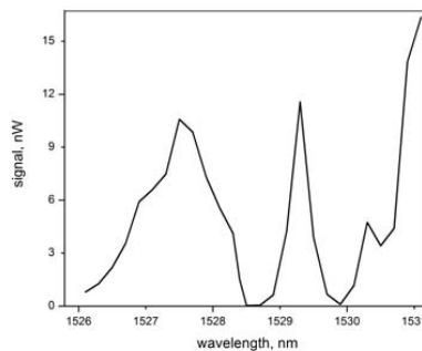
Fig. 2. Transmission spectrum of FPI, utilizing Si-on-LiNbO 3 structure. Attenuation of signal in wavelength range between 1526 and 1527.5 nm is caused by sharp decrease of output power of tunable light source at low limit of working range.
