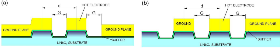
Figure 1: Cross section of the CPW structure on ridge (a) and the new proposed SCCPW (b).
