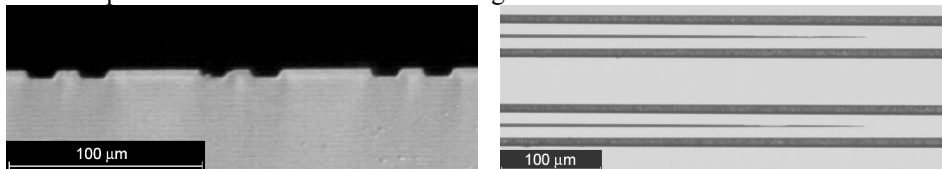
Figure 4: Fabricated end faces of the modulator ridge waveguides (left) and Y-splitters (right).
