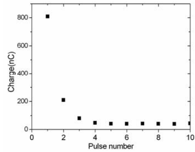
Fig. 6: The accumulated charge per rectangular poling pulse of 270 V as function of the pulse number.
