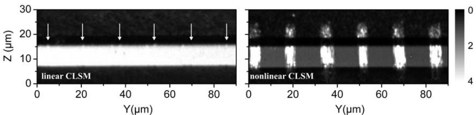
Fig. 7: Linear CLSM image of the X-face of a 10 \mu\text{m} wide ridge of 2.0 \mu\text{m} height; the faint periodic edge modulation is indicated (left). SH-signal generated by the nonlinear CLSM from the same surface (right). A grey scale of both, the fundamental- and SH-intensities, is given on the right.
