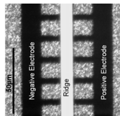
Fig. 4: Top view (optical micrograph) of the electrode structure of 16.6 \mu m periodicity on both sides of a 10 \mu m wide ridge.
