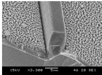
Fig. 2: SEM micrograph of an etched ridge of 5.8 \mu\text{m} height and 5.0 \mu\text{m} width on X-cut LN.
