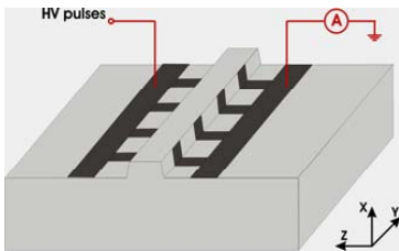
Fig. 3: Scheme of the poling configuration for a ridge on X-cut LN.
