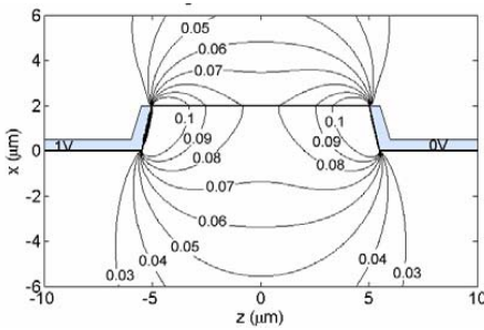
Fig. 5: Calculated lines of constant E_z (in MV/m) in a ridge of 2.0 \mu\text{m} height and 10 \mu\text{m} width, assuming 1 V applied to the left electrode.
