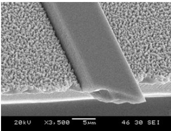
Fig. 1: SEM micrograph of an etched ridge of 2.4 \mu\text{m} height and 9.0 \mu\text{m} width on X-cut LN.
