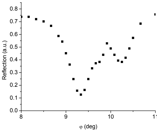
Figure 5: Reflection near the resonance
