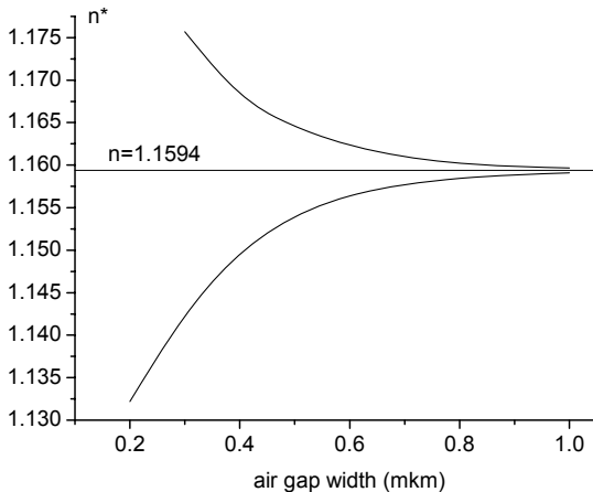
Figure 6: Effective indices of two surface waves
