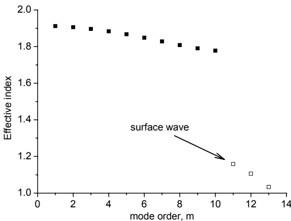
Figure 1: modes of the waveguide structure
