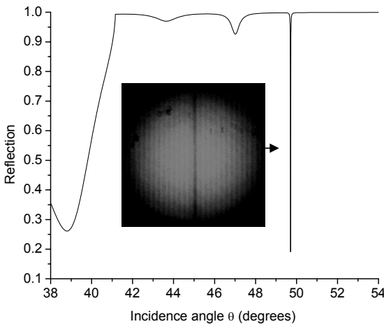
Figure 3: Reflection from the single structure
