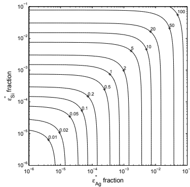
Figure 3: Contour plot of the loss values in \text{dB}/\mu\text{m} when the \epsilon'' values of both Ag and Si are varied in fractions of their natural values at room temperature.
