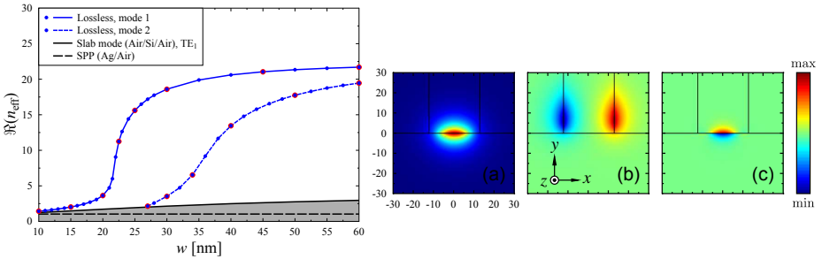
Figure 2: Left panel: Geometric dispersions of first two modes of the waveguide with respect to w . Loss is assumed to be zero. Red dots: the n_{\text{eff}} values when \epsilon'' values of both Ag and Si are reduced to their 1%. Right three panels are field plots of the waveguide with a 25nm-sized core: (a) H_x field (min:0, max:1.27); (b) H_y field (min:-5.02e-2, max:5.02e-2); and (c) z -component Poynting vector S_z (min:-6.0e2, max:6.2e2). Axis unit: nm.
