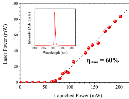
Fig. 3: Experimental output efficiency curve. The inset shows the laser line, obtained for TM excitation at 748 nm.
