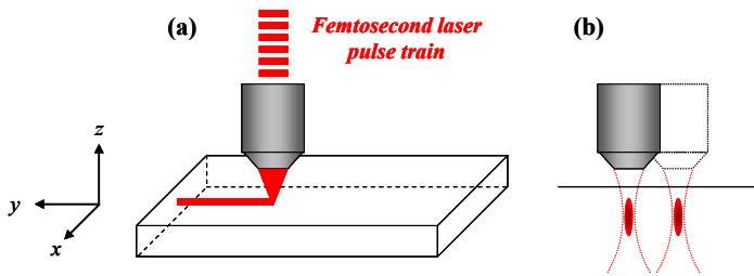
Fig. 1: (a) Diagram showing the direct laser writing of waveguides by using a femtosecond laser. (b) Two parallel lines, separated 20 \mu\text{m} , were written by translating the sample in the x-direction.
