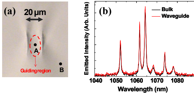
Fig. 2: (a) Optical transmission image of the end face, the guiding region has been indicated. (b) {}^4F_{3/2} \rightarrow {}^4I_{11/2} \text{Nd}^{3+} emission band measured at the waveguide and at the bulk, points A and B in Fig. 2(a), respectively.
