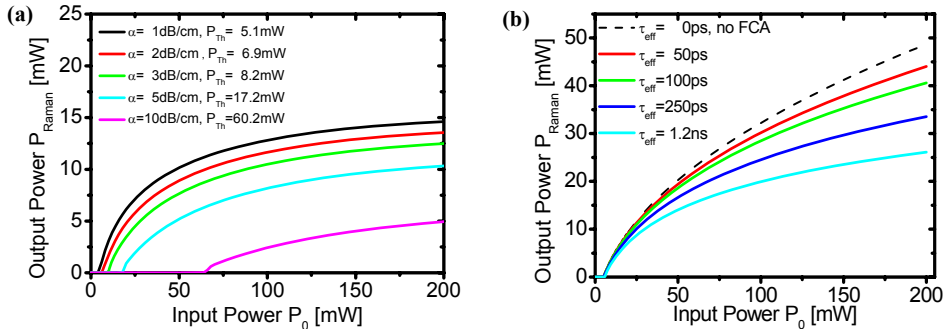
Fig. 3: (a) Raman output power P_{\text{Raman}} vs. input pump power P_0 for different linear propagation losses \alpha = \alpha_p = \alpha_s and \tau_{\text{eff}} = 1.2 ns. (b) Raman output power P_{\text{Raman}} vs. input pump Power P_0 for different effective carrier lifetimes \tau_{\text{eff}} and \alpha = 2 dB/cm.
