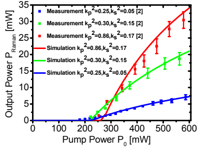
Fig.2: Output power Raman laser over input pump power. Shown are the experimental data taken from Ref. [2] and our simulation results (solid lines) for different coupling coefficients \kappa_{p/s}^2 .
