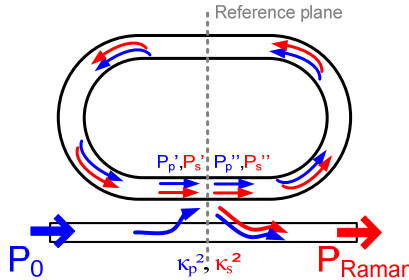
Fig.1: Schematic view of a racetrack resonator. P_0 represents the initial pump power, P_{\text{Raman}} the output power of the Raman laser at the Stokes wavelength \lambda_s . \kappa_{p/s}^2 describe the wavelength dependent coupling coefficients between bus waveguide and resonator.
