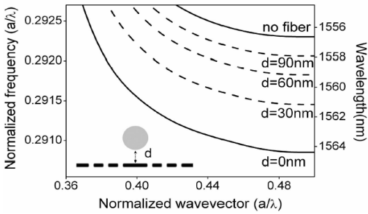
Fig. 3 Dispersion curve of fiber-coupled PhC waveguide.
