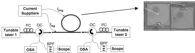
Fig 1. Experimental set-up for SRL characterization. Chip top-view and ohmic contacts are also reported.
