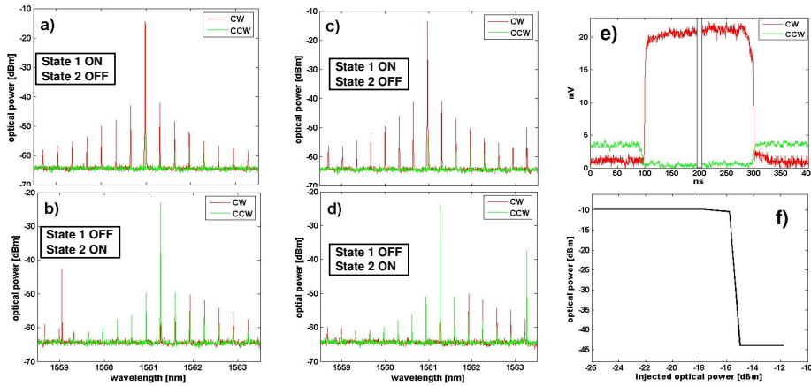
Figure 3. a-d) Optical spectra of the CW and CCW modes for injected signal at different wavelengths. e) Time domain traces showing the switching between bistable states. f) Optical transfer function of state 1 (state 2) as function of the optical input power of the set (reset) signal.
