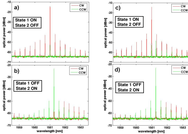
Figure 2. Optical spectra of the CW and CCW modes at different memory states.
