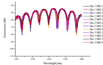
Fig.3 Spectral response of 12 MZI's from 3 different Dies
