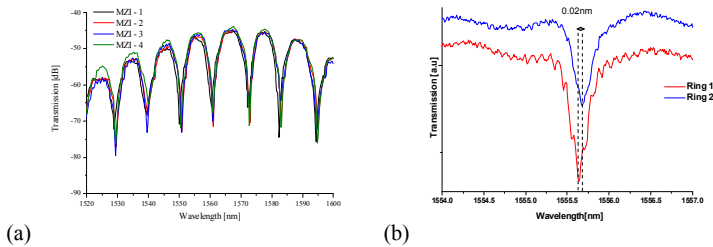
Fig. 2 (a) Spectral response of 4 MZI's within a die, (b) Spectral response of two racetrack ring resonators which are 25µm apart.
