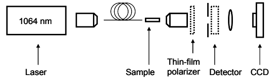
Fig. 1: Experimental set-up for waveguide transmission measurements and mode analysis.
