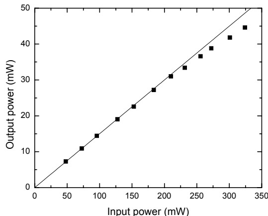
Fig. 4: Non-linear transmission through a 5-mm long nanowire waveguide. At high input powers, absorption in the waveguide core results in a heating of the waveguide which lowers its effective index and reduces the transmitted power.
