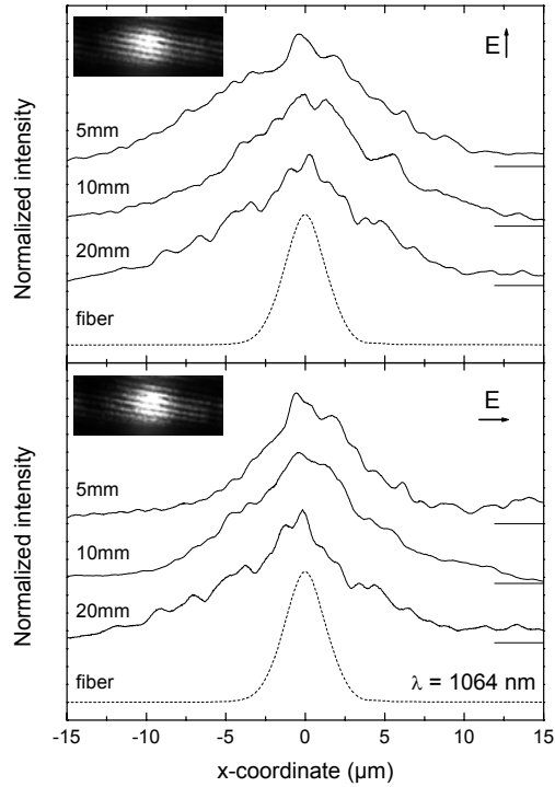
Fig. 2: Mode profiles recorded of at the output facets of nanowire waveguides samples of different lengths for orthogonal input polarizations. Irregularities in the intensity plots are due to dicing marks on the facet, as seen in the inset figures. The fiber mode is shown for reference.
