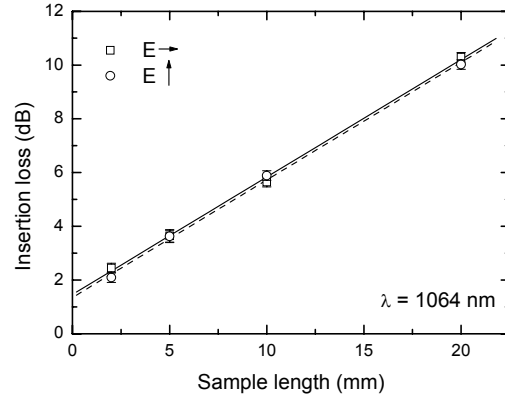
Fig. 3: Cutback measurements on nanowire waveguides for different input polarizations. The solid and dashed lines show the least-squares fit to the data points for horizontally and vertically polarized input fields, respectively, giving a propagation loss of 0.43 dB/mm for both polarizations.
