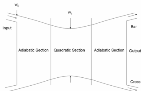
Fig. 5: 2x2 hybrid splitter showing the adiabatic and quadratic sections.
