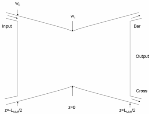
Fig. 2: 2x2 adiabatic MMI splitter showing the input and output waveguides
