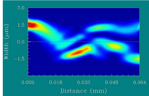
Fig. 3: BPM simulation of propagation through an adiabatically tapered 2x2 MMI splitter.
