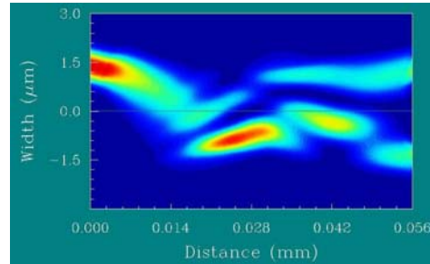
Fig. 3: BPM simulation of propagation through a hybrid tapered 2x2 MMI splitter.
