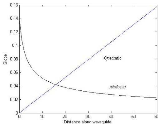
Fig. 4: Comparison of slopes of quadratic and adiabatic half-profiles where n_1 = 3.32517 , n_2 = 3.17 , \lambda_0 = 1.507
