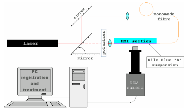
Fig.1 Experimental arrangement
