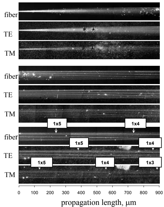
Fig.4 The successive sequences of recorded mode field interference images for MMI section of the width 60 \mu\text{m} , excited at 1/3 rd of the section width.
