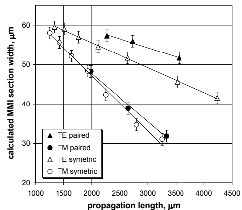
Fig.7 The dependence of calculated MMI section width on the propagation length for MMI section of the width 60\ \mu\text{m} .
