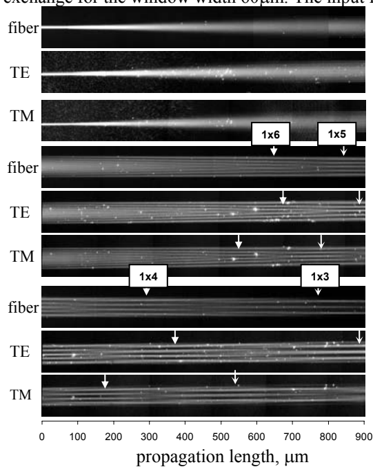
Fig.3 The successive sequences of recorded mode field interference images for MMI section of the width 60 \mu\text{m} symmetrically excited (a)
