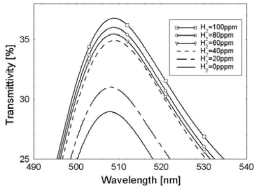
Fig.2: Transmission spectra for the optimized H 2 sensor: an increase of 7.4% in terms of transmittivity is noticed when a malabsorption condition occurs, i.e. the overtaking of the 20ppm baseline; the total increase of the transmittivity swelling the hydrogen concentration from 20ppm to 100ppm is about 15.6%.
