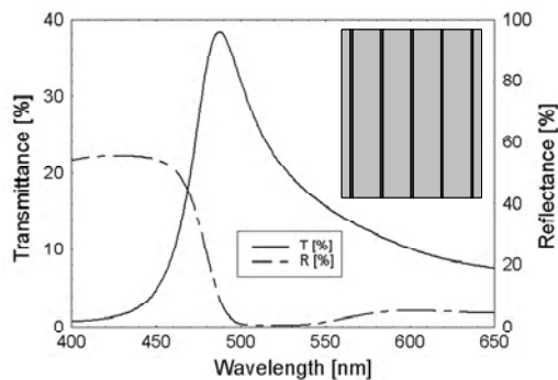
Fig.1: Sketch of transmission and reflection spectra for the multilayer structure. The inset shows the sensor structure: light grey regions are the dielectric layers (EXP0454) and dark grey regions are the metal layers (Pd).
