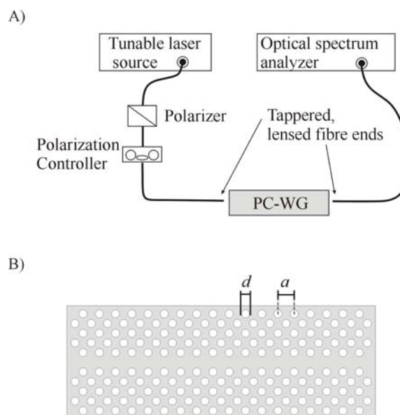
Fig. 1: A) Experimental setup. B) Top-view of the photonic-crystal waveguide configuration.
