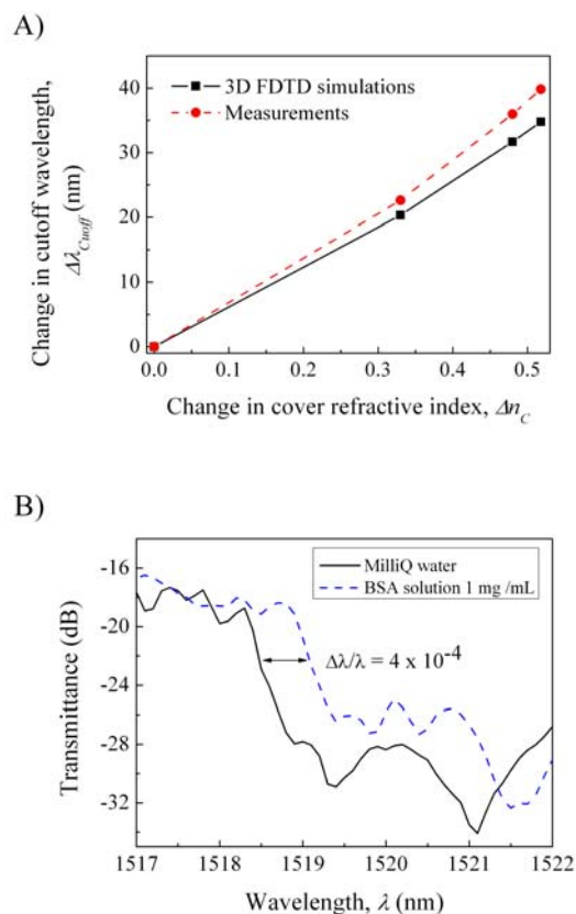
Fig. 2: (A) Curves showing the experimental (circles, dashed line) and simulated (squares, solid line) changes in wavelength position of the band-gap edge vs. changes in cover RI. (B) Measured curves before (solid line) and after (dashed line) protein adsorption on the sensor surface.
