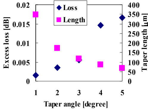
Fig. 3: Excess loss and taper length as a function of taper angle.
