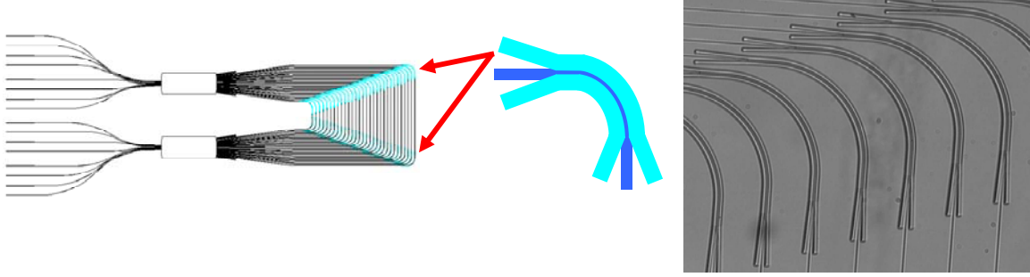
Fig. 6: Schematic of a 90 degree AWG using trenches filled with low-refractive index material.
