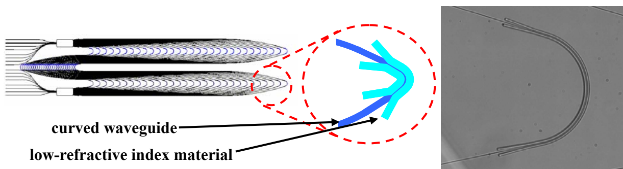
Fig. 8: Schematic of the triple arrowhead type AWG using trenches filled with low-refractive index material.
