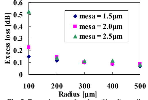
Fig. 5: Excess loss as a function of bending radius.
