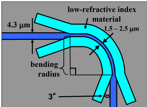
Fig. 4: Schematic of a 90-degree bend waveguide for calculating bending loss.
