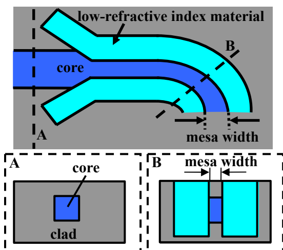
Fig. 1: Schematic of a silica bend waveguide with trenches filled with a low-refractive index material.
