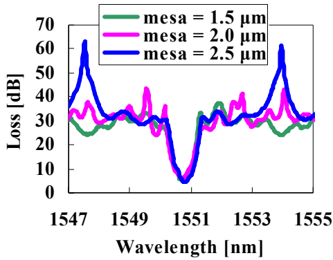
Fig. 7: Transmission characteristics from the center port of a 90 degree bend AWG.
