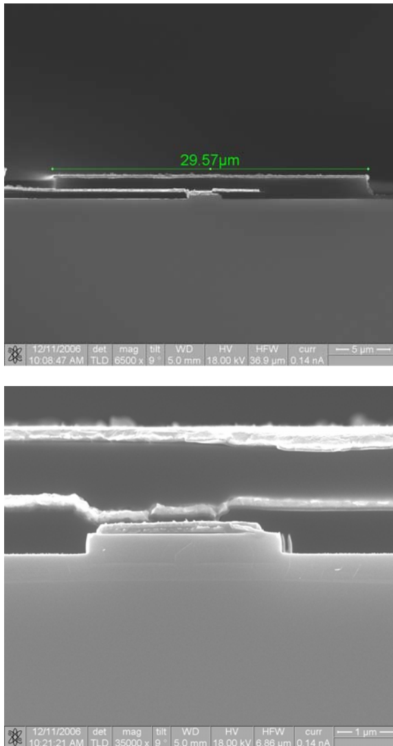
Fig. 3: SEM pictures of the cross-section of the amplifying waveguide optical isolator with integrated electromagnet.
