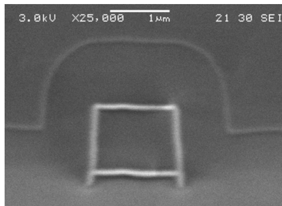
Fig. 1: Photograph of a box-shaped waveguide realized with TriPleX technology. The clear box is \text{Si}_3\text{N}_4 65nm thick; the gray surrounding is \text{SiO}_2 .
