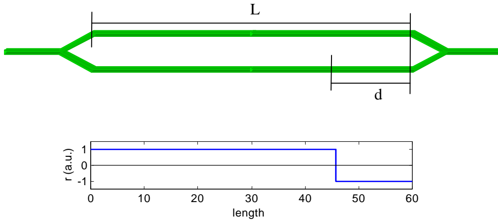
Fig. 1 Mach-Zehnder intensity modulator with double-domain inverted structure. L is the modulator length and d the last section with opposite domain orientation.
