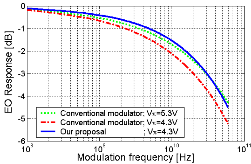
Fig. 2 Comparison between our proposal and conventional modulators in terms of EO response
