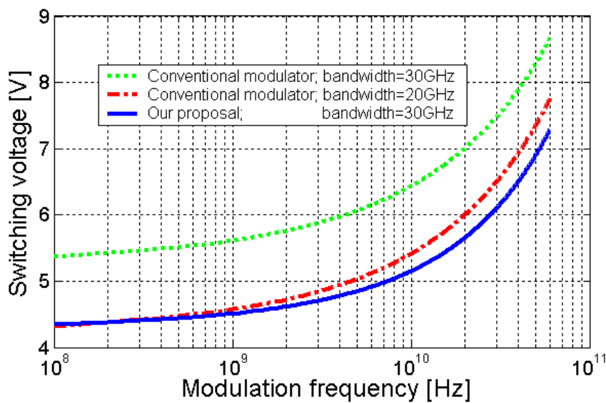
Fig. 3 Comparison between our proposal and conventional modulators in terms of V_p
