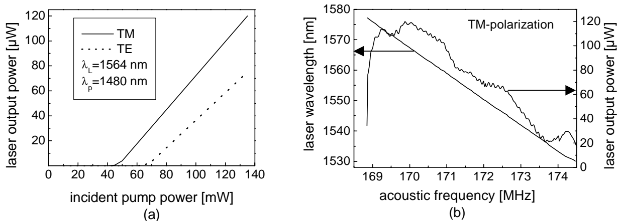
Fig. 2: (a) Laser output power versus incident pump for two modes of operation in TM- and TE-polarization, respectively. (b) laser emission wavelength (left ordinate) and output power (right ordinate) versus SAW-frequency at 135 mW of pump power in TM-mode of operation.
