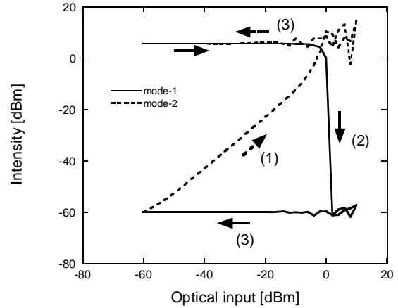
Fig. 4 Bistable switching characteristics of the MMI-BLD.
